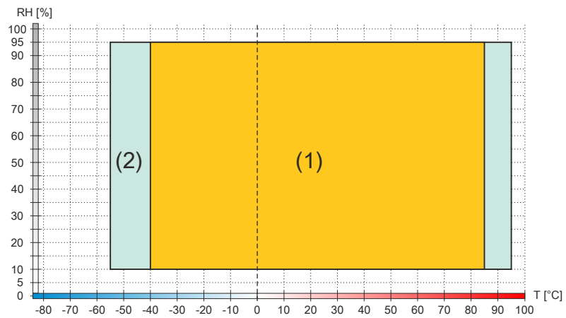
Figure 2: 5MMSSD.0512-00 - Temperature/Humidity diagram - Up to Rev. C0
