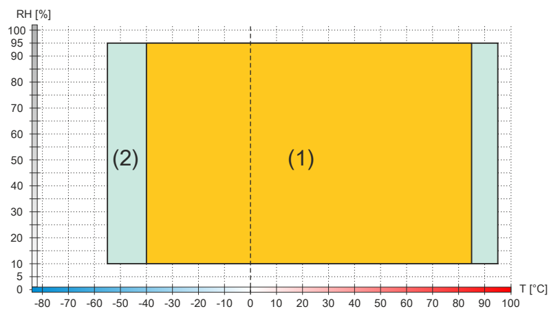
Figure 1: 5MMSSD.0512-00 - Temperature/Humidity diagram - Rev. D0 and later
